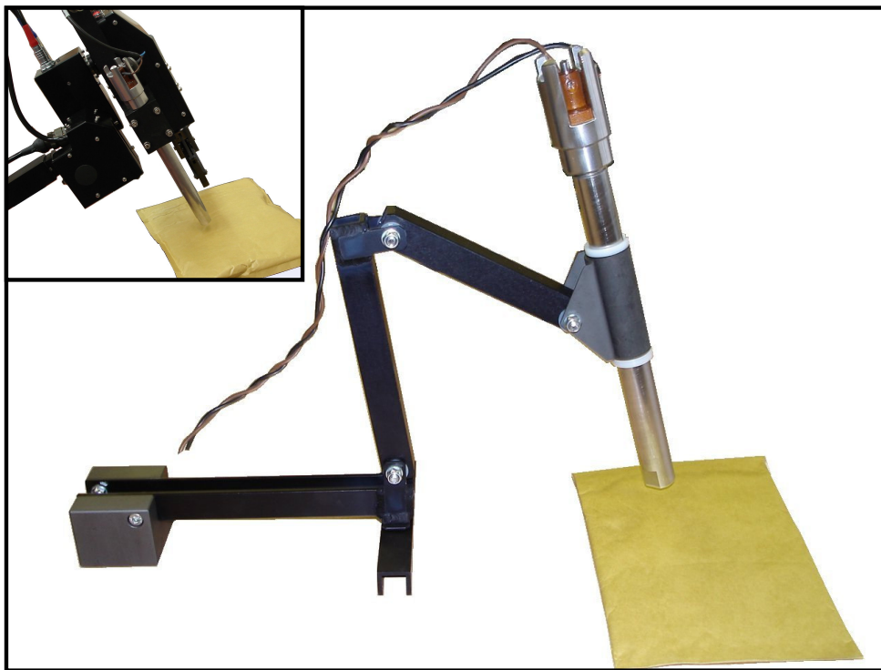
Needle shown deployed using the supplied stand and mounted on Cyclops ROV (inset)
